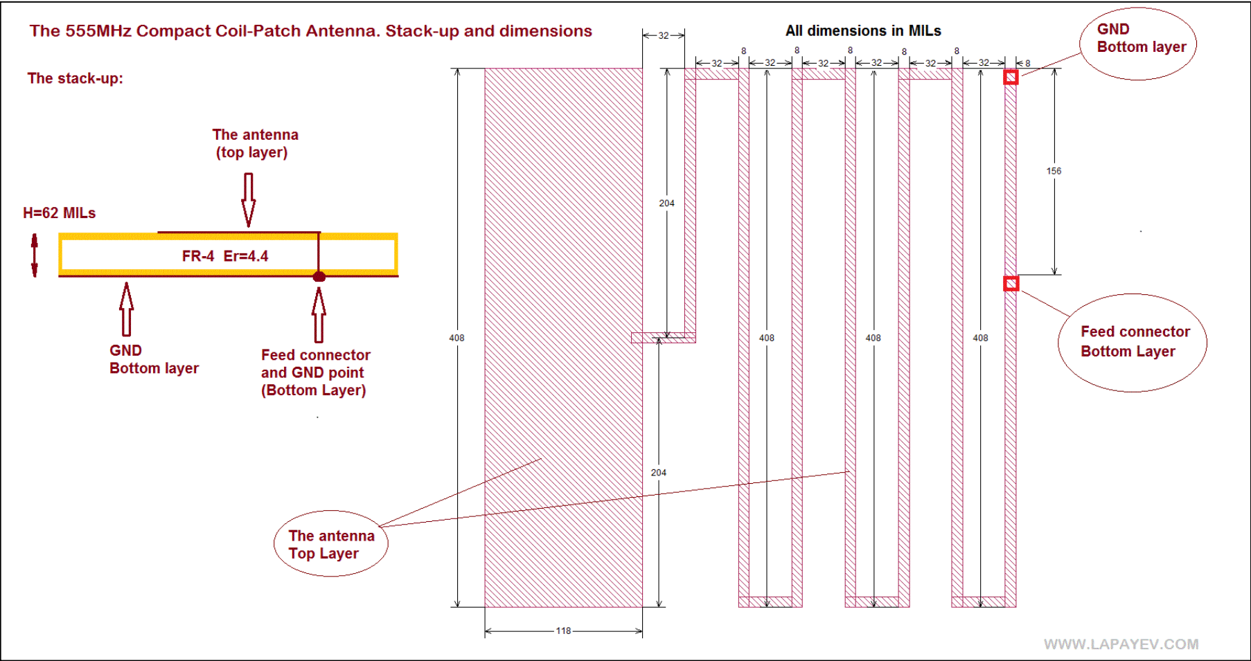
2. 555 MHz antenna. The design and dimensions.
