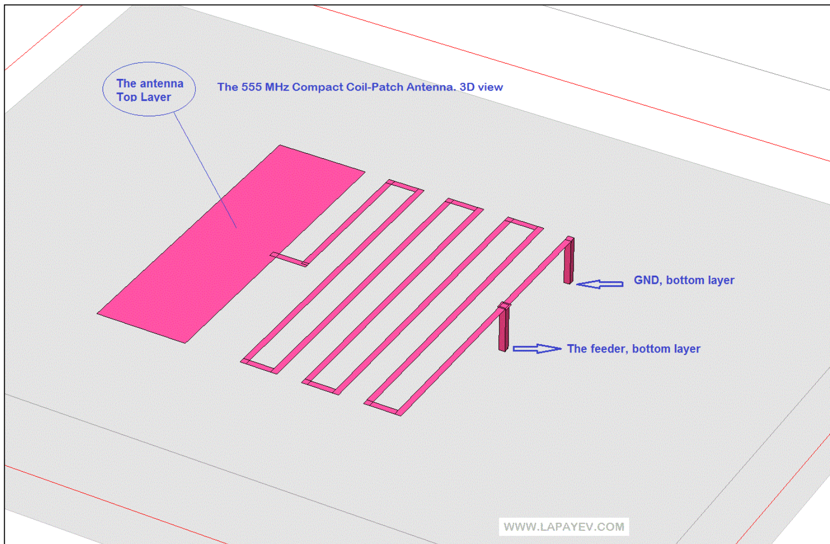
1. 555 MHz antenna. The 3D view
