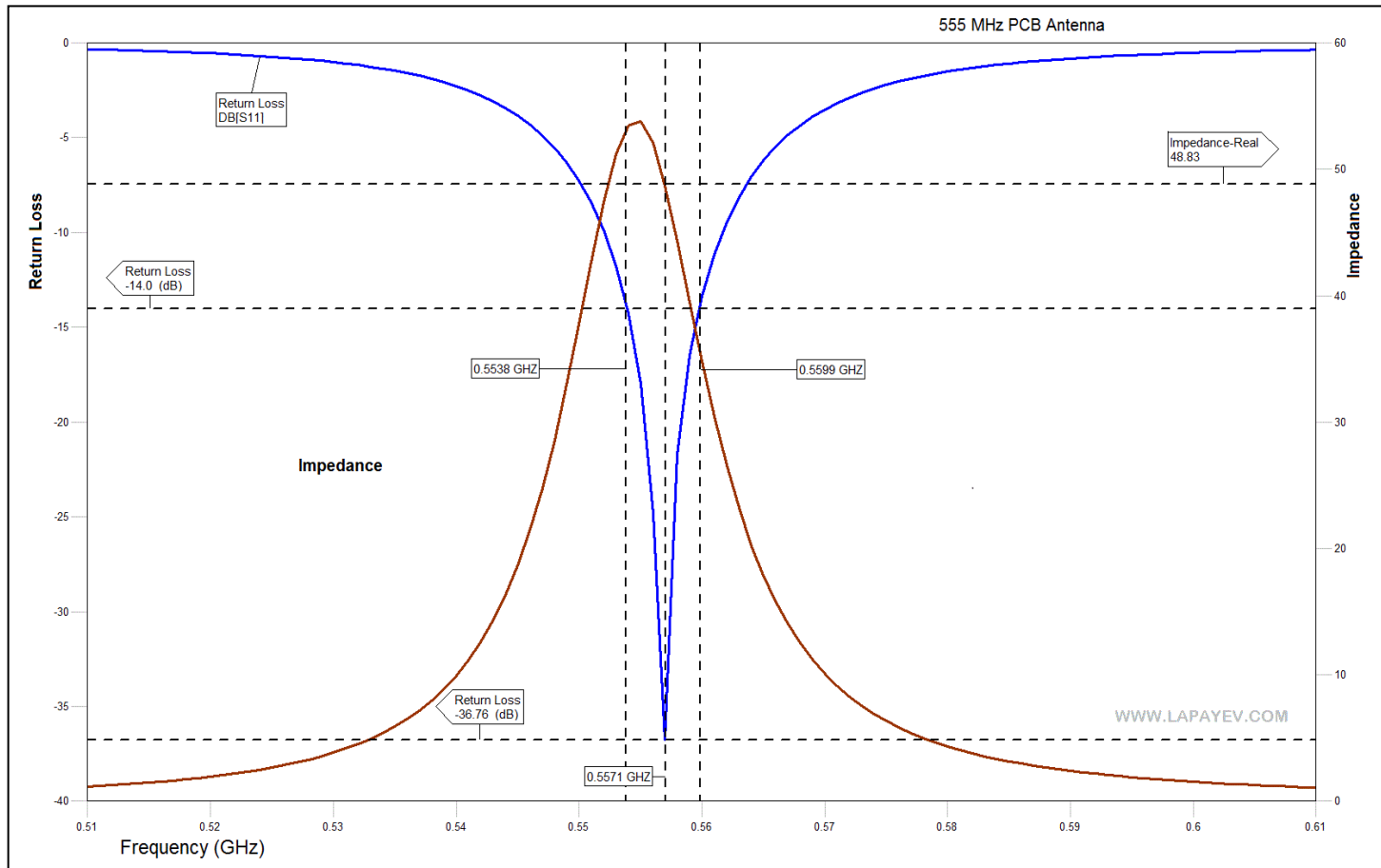
1. 555 MHz antenna. 555 MHz antenna. The Return Loss and Impedance.
