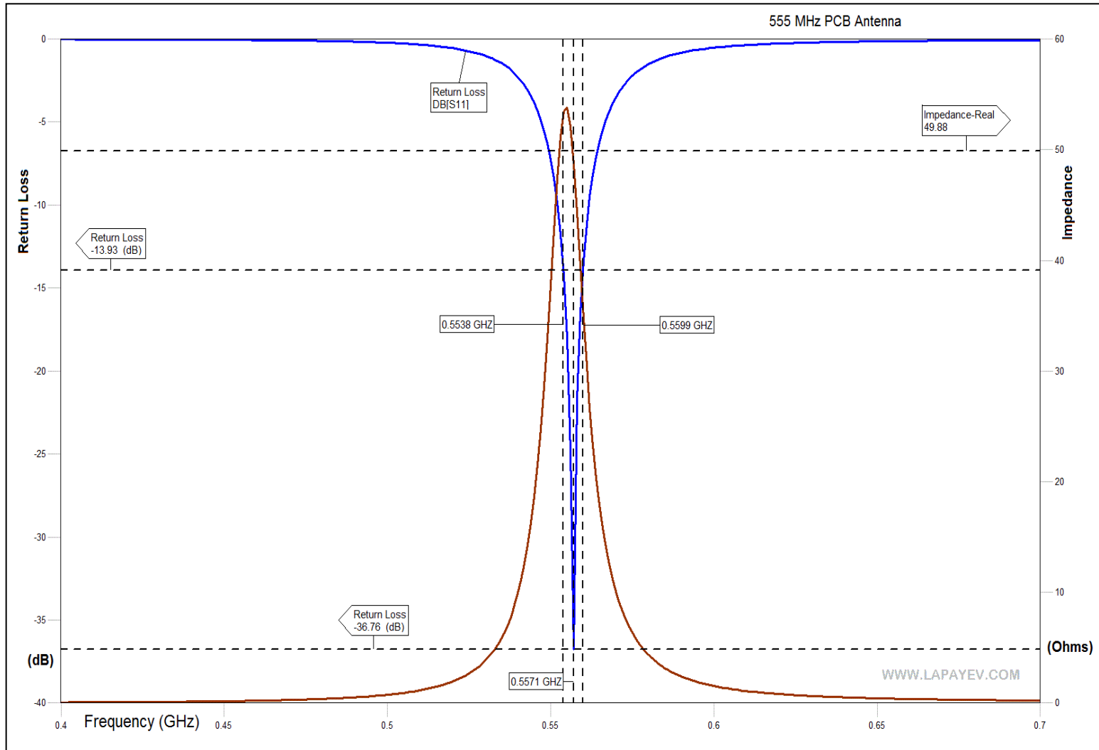
3. 555 MHz antenna. The Return Loss and Impedance.
