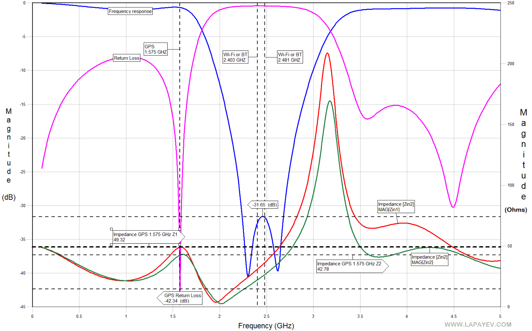
GPS 1.57542 GHz. Bluetooth and Wi-Fi PCB notch filter 2.4GHz
